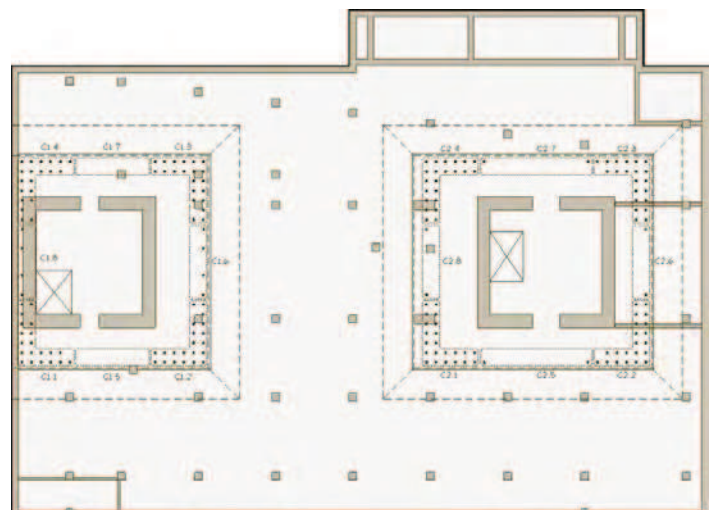
Figure 7: Plan view of hybrid mat slab foundation showing micropile clusters
