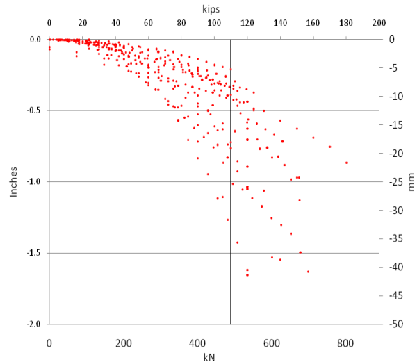
Figure 7. 1¾" (44 mm) Square shaft load test data
