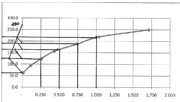
Figure 10. Illustration of Mazurkiewicz's method
