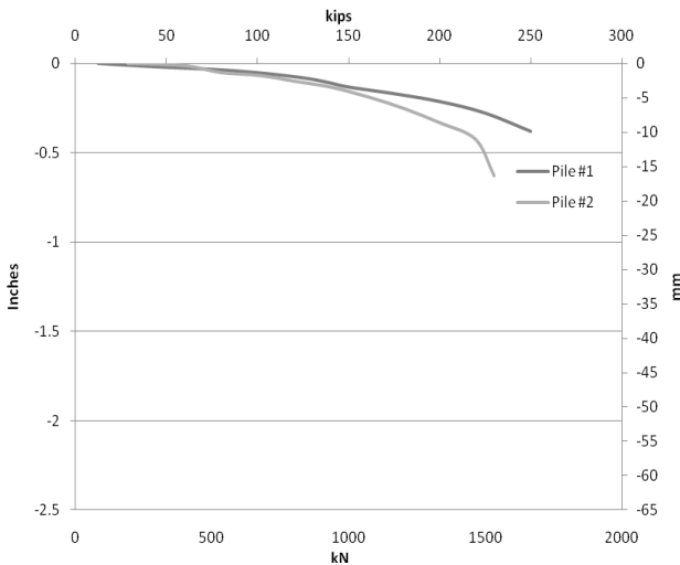
Figure 5. 2-¼" (57 mm) Piles #1 and 2 load test data
