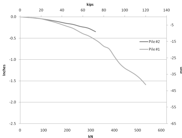
Figure 2. 1½" (38 mm) Piles #1 and 2 load test data
