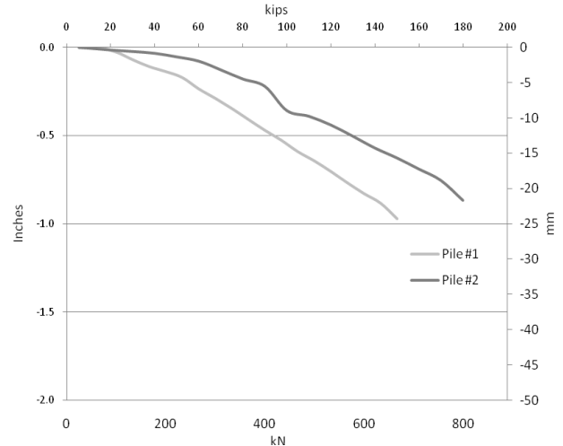
Figure 3. 1¾" (44 mm) Piles #1 and 2 load test data
