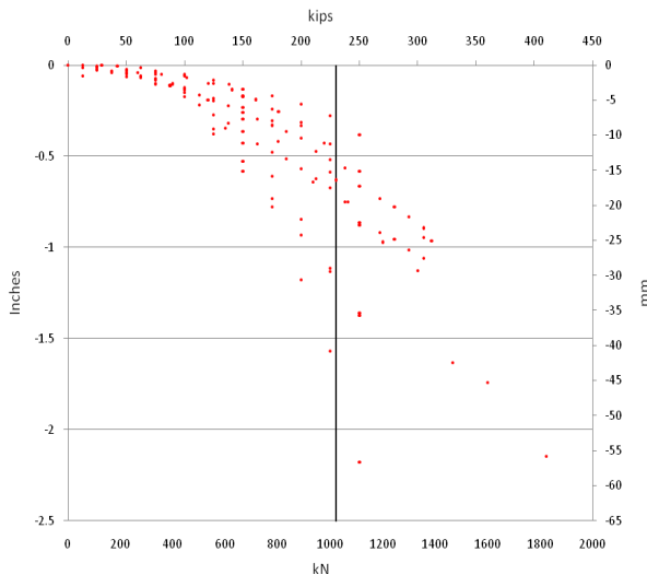
Figure 9. 2 1/4" (57 mm) Square shaft load test data
