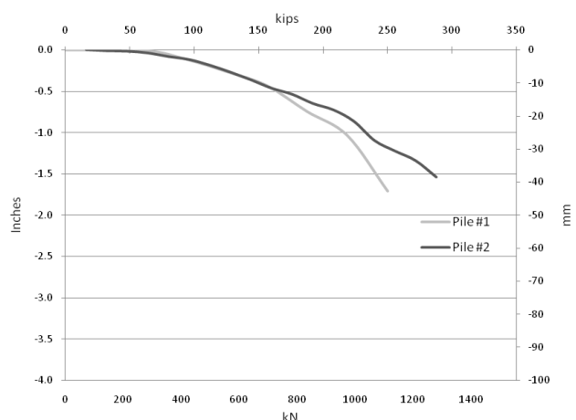
Figure 4. 2" (51 mm) Piles #1 and 2 load test data
